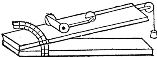
INCLINED PLANE AND CARRIAGE.
